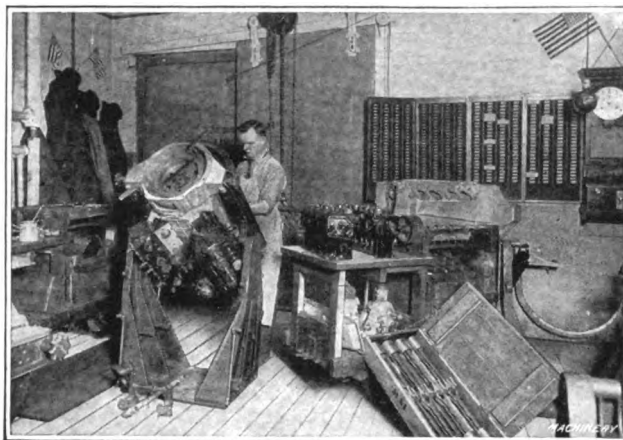
Fig. 9—Time is often lost through assemblers having to make trips to the storeroom to obtain missing parts. The Cadillac Motor Car Co. has overcome this difficulty by constructing trucks with individual compartments for carrying a complete set of parts for a motor
